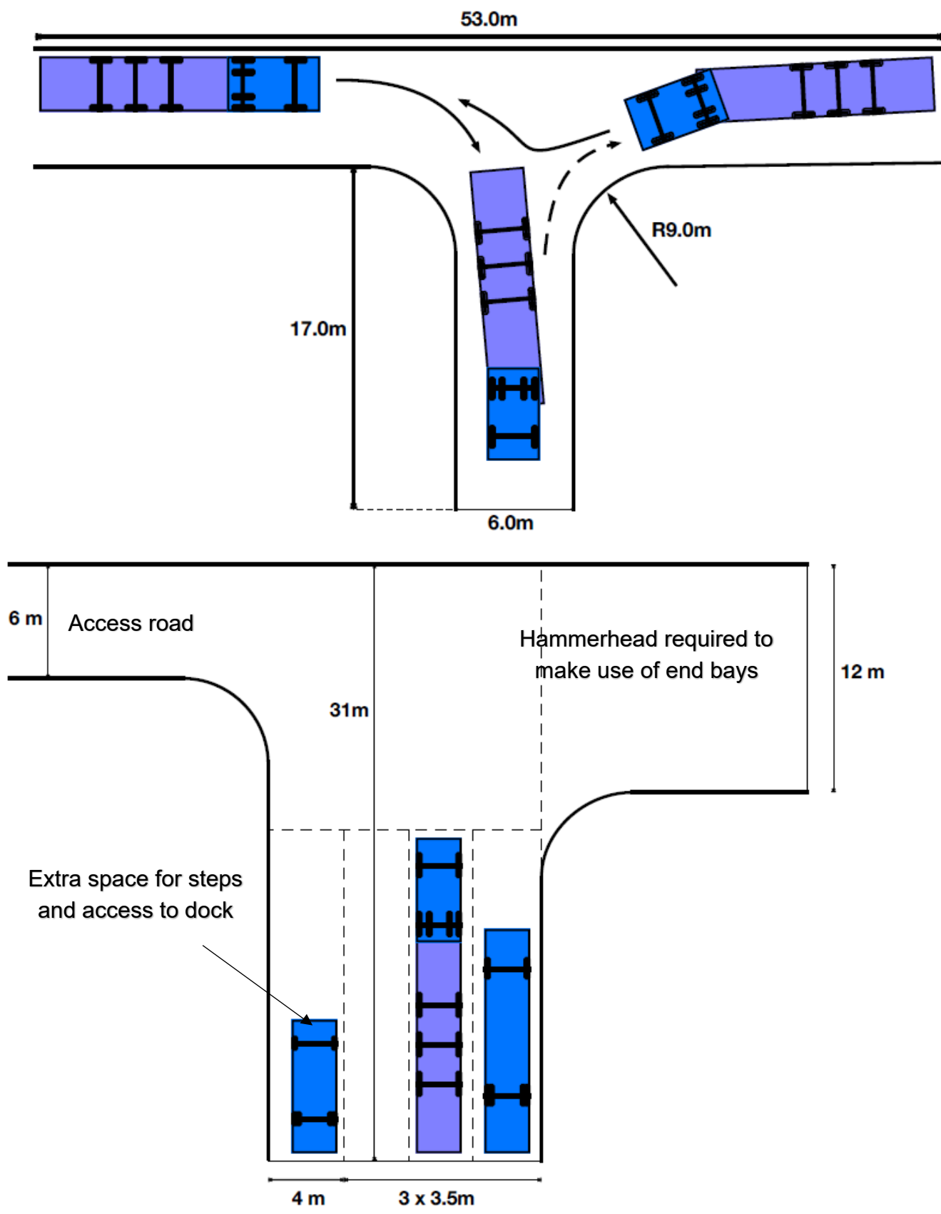
Figure 3.2.11 Service yard T-turning area – design artic, 40 tonne gross vehicle weight, 16.5m long, 2.55m wide
