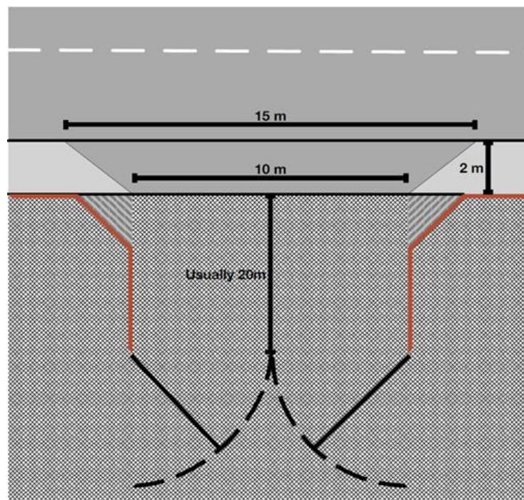
Figure 3.2.6 Dropped kerb (industrial access)
