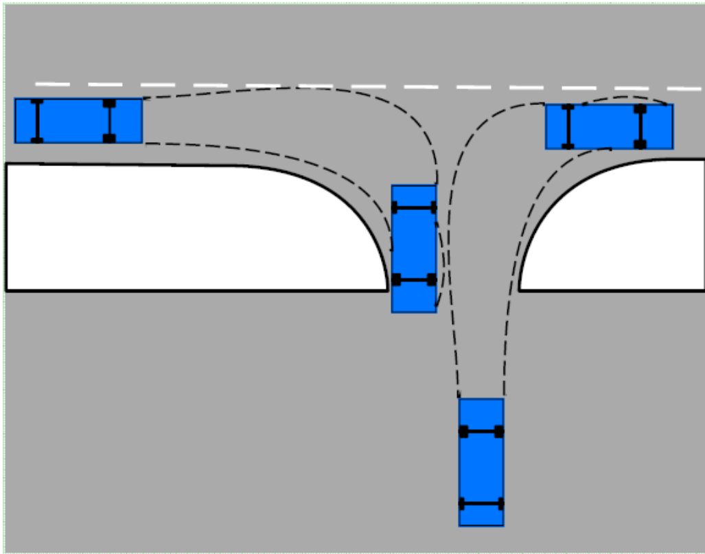
Figure 3.2.1 Simple turn
