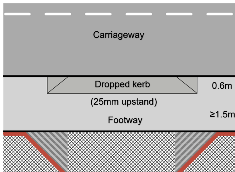
Figure 3.2.4 Dropped kerb (small scale commercial development)
