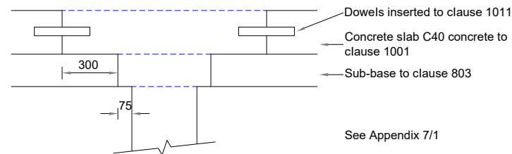
REINSTATEMENT OF CARRIAGEWAY WITH UNREINFORCED CONCRETE SLAB
