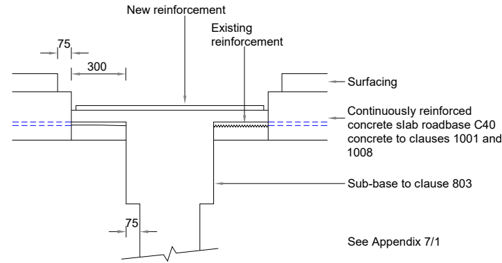
REINSTATEMENT OF CARRIAGEWAY WITH REINFORCED CONCRETE ROADBASE
