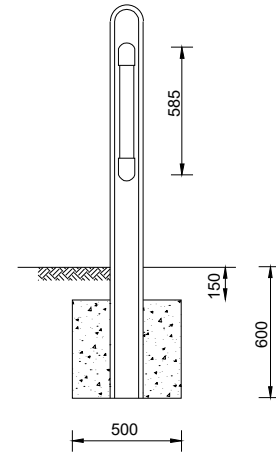
FOUNDATION DETAIL
