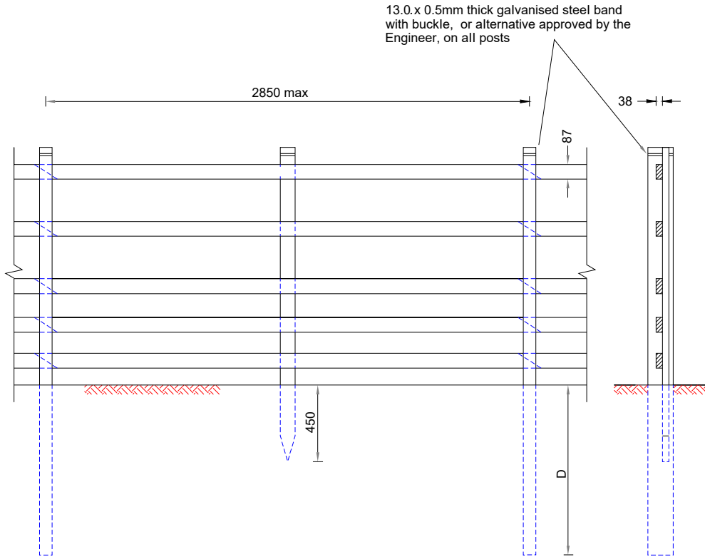
TYPICAL CONSTRUCTION DETAILS - MORTICED POST AND FIVE RAIL FENCING
