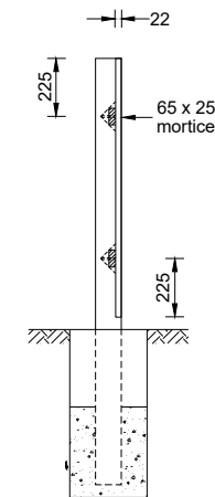
ELEVATION OF WOODEN POST REF WPW 105
