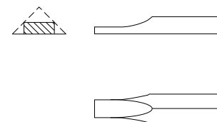
SHAPING OF ARRIS RAILS FOR MORTICE
