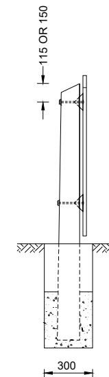
ELEVATION OF CONCRETE POST REF WPC 105
