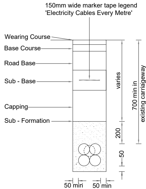
1, 2, 3 OR 4 WAY DUCTS IN CARRIAGEWAY
