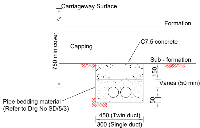
DUCTS LAID PRIOR TO CAPPING
