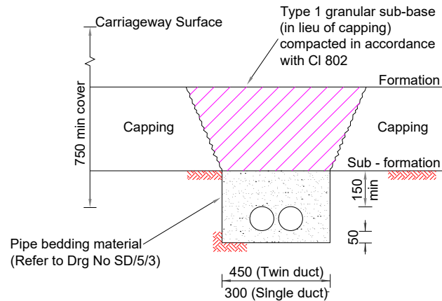
DUCTS LAID AFTER CAPPING OR IN EXISTING CONSTRUCTION
