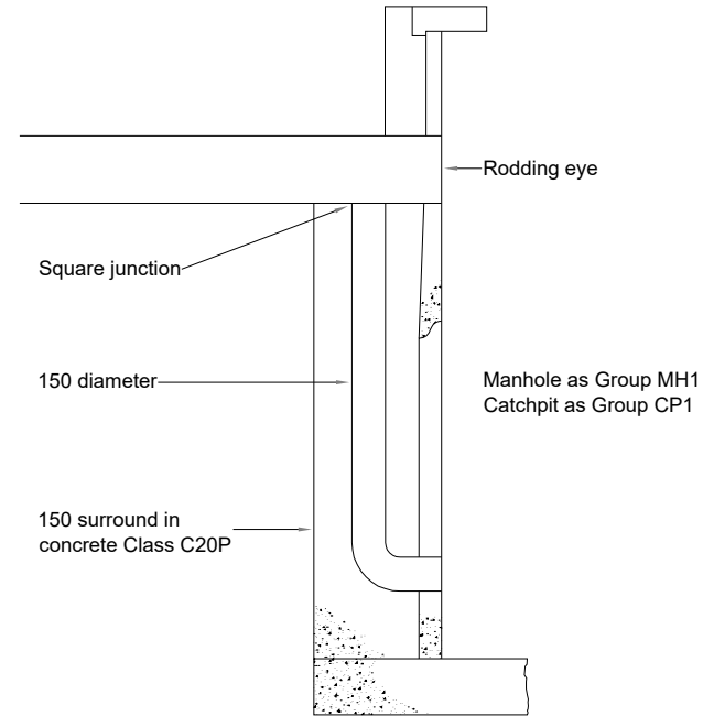
TYPE 2 - BACKDROP GREATER THAN 2m
