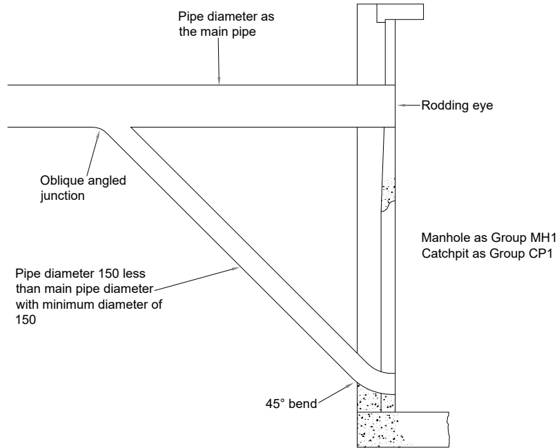
TYPE 1 - BACKDROP LESS THAN 2m
