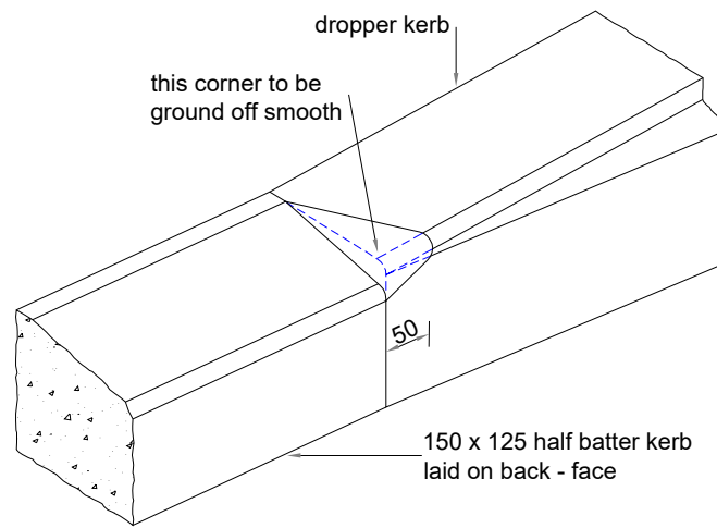
Kerb detail
