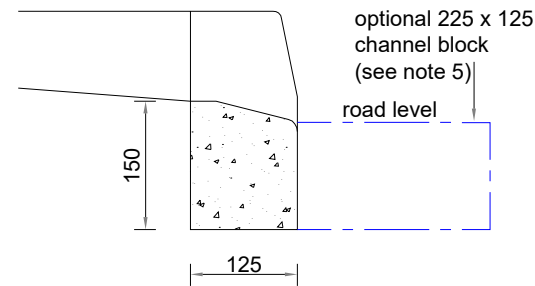
Cross section
