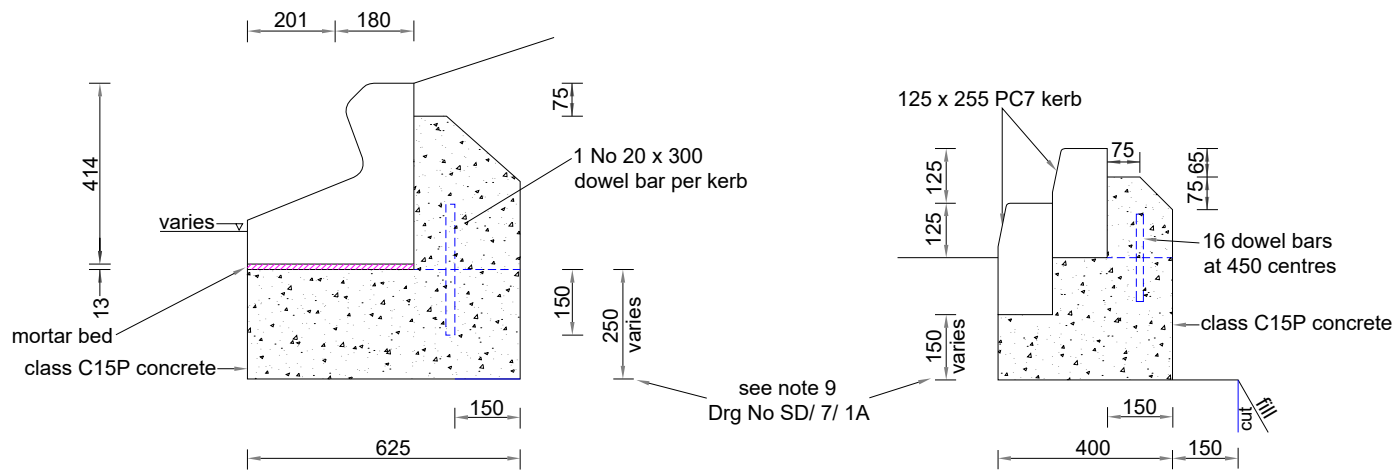
Double kerb - K19
