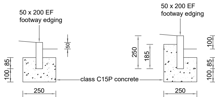
Footway edging EF 200
