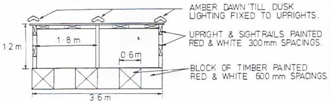
ELEVATION - SCALE 1:5
