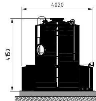
WEST Scale 1:100
