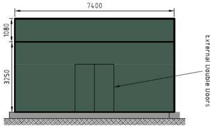
SOUTH Scale 1:100
