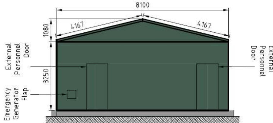
WEST Scale 1:100
