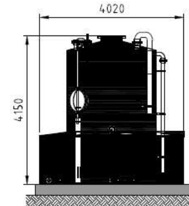
SOUTH Scale 1:100
