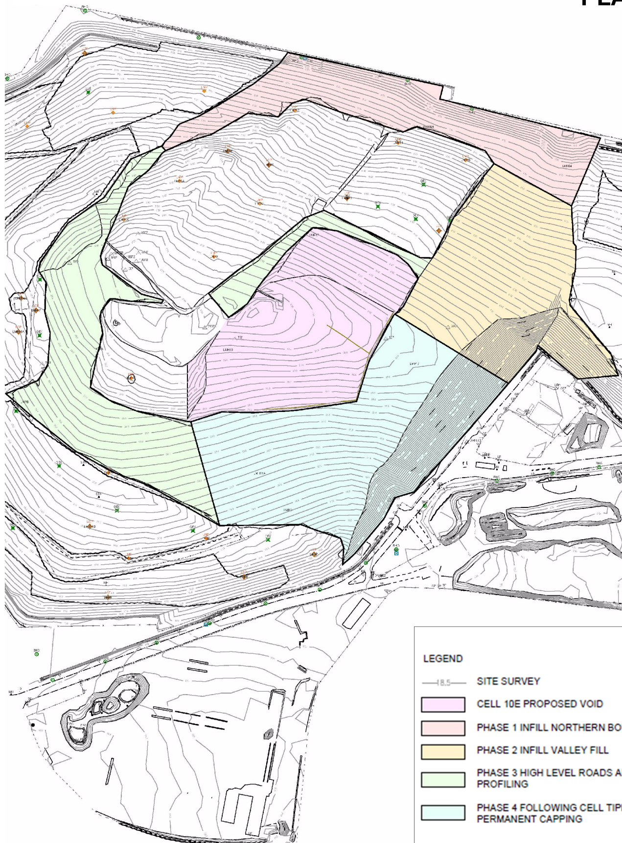
PLAN SHOWING SOILS INFILL TO RESTORATION – 444,925m 3 NTS
