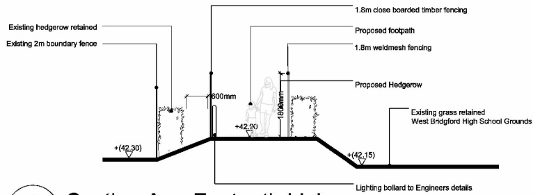
A Section Aa - Footpath Link 1:50
