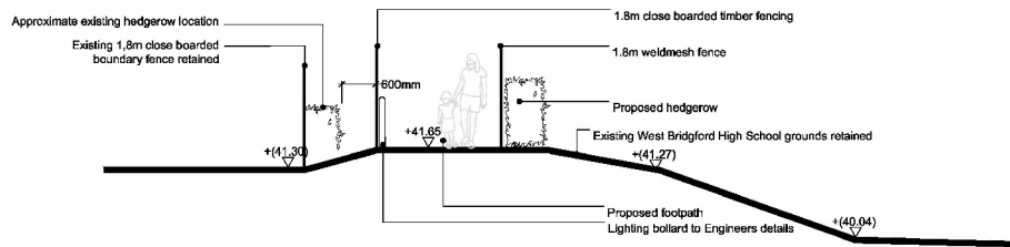
B Section Bb - Footpath Link 1:50
