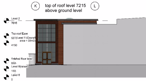
3 KS2 Proposed West Elevation 1: 100
