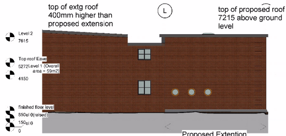
2 KS2 Proposed East Elevation 1: 100
