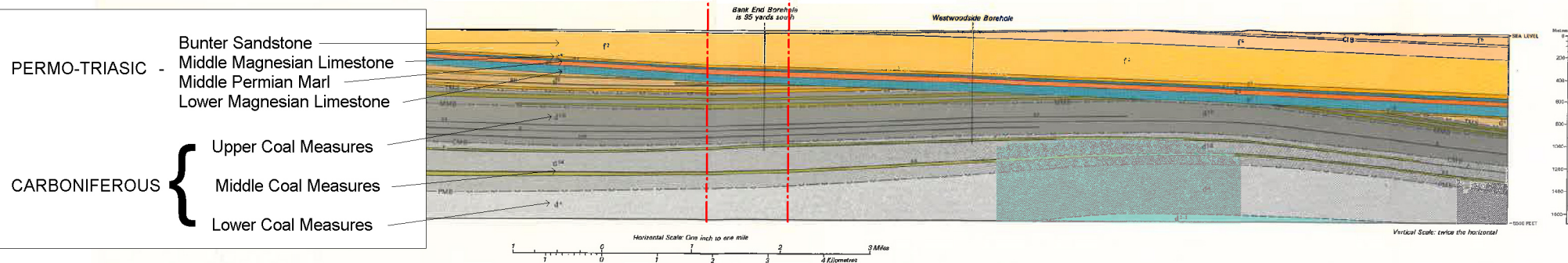
SECTION SHOWING THE GENERAL RELATIONS OF THE SOLID ROCKS ALONG THE SAME LINE AS ABOVE
