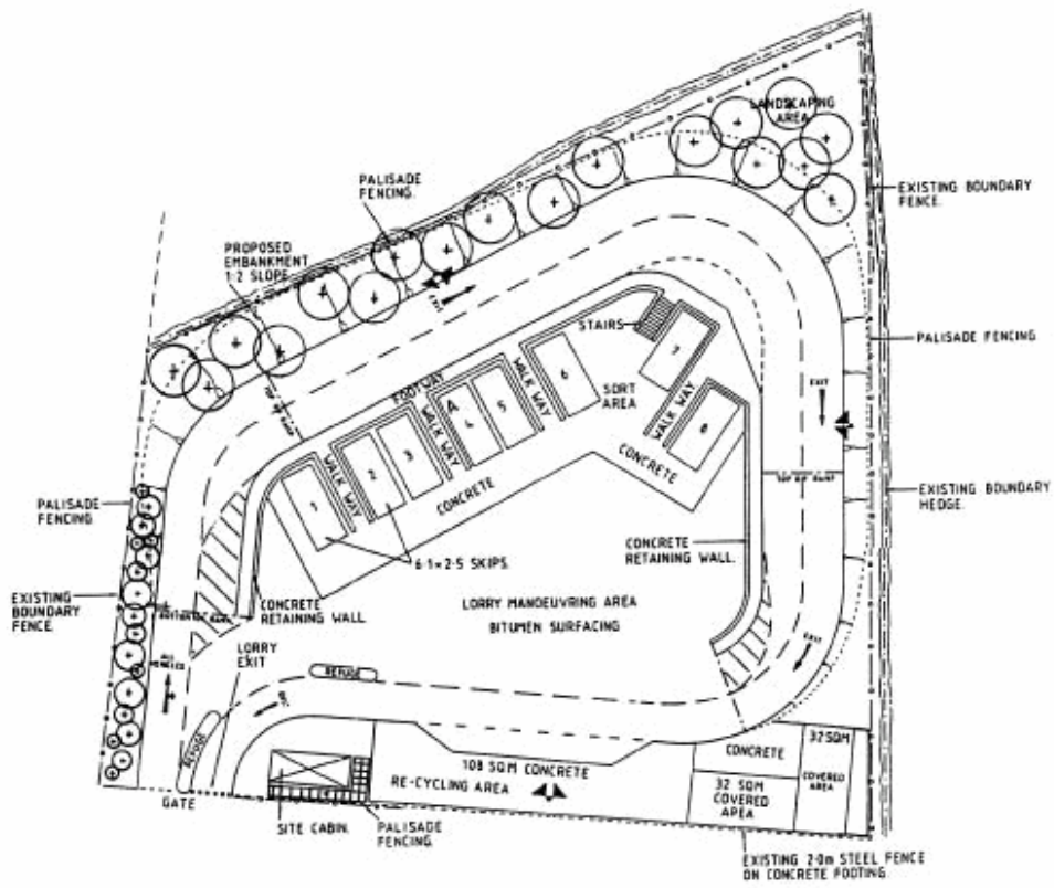
Figure 5.2 - Illustration of a Typical HWRC.
