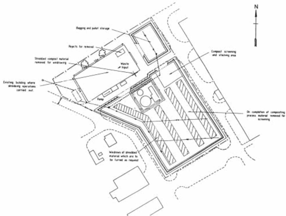
Figure 7.1 - Diagram of Langar Composting Scheme (Extract from Planning Application, Courtesy of Waste Recycling Group)
